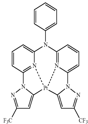
Compound 249 described in JP-A-2007-19462
