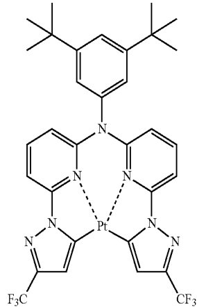
Compound 255 described in JP-A-2007-19462
