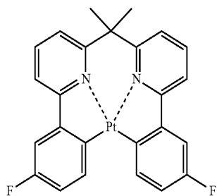
Compound 34 described in JP-A-2006-93542
