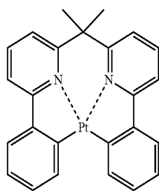
Compound 79 described in JP-A-2005-310733
